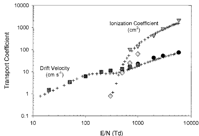
FIG. 6. Calculated drift velocities V_d and ionization coefficients \alpha/N for electrons in TEOS. The filled squares are V_d calculated using a numerical solution of Boltzmann's equation. The filled circles are results of Monte Carlo simulations. The diamonds are \alpha/N from solving Boltzmann's equation and the triangles are the Monte Carlo results. Experimental values 14 are shown by the + signs.
