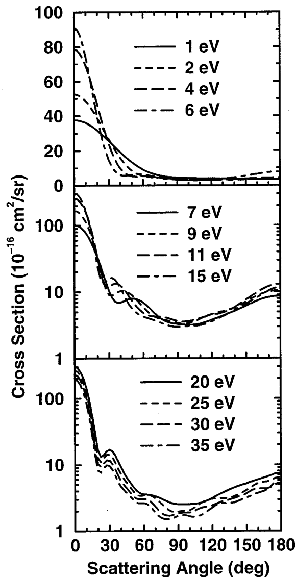
FIG. 2. Elastic differential cross section for scattering of electrons by TEOS at representative energies.
