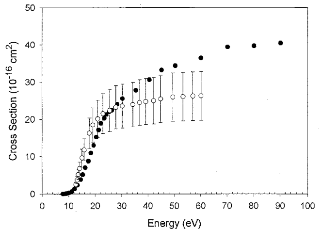
FIG. 3. Electron-impact total ionization cross sections for TEOS. The open circles with error bars are the measurements of Holtgrave et al. , 6 and the solid circles are those of Basner et al. 7
