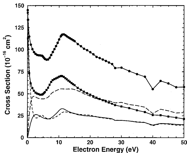
FIG. 1. Integral elastic cross section (solid line with circles) and momentum-transfer cross section (solid line with squares) for electron scattering by TEOS. Also shown are the symmetry components of the integral cross section: dotted line, {}^2A ; solid line, {}^2B ; dashed line, {}^2E .
