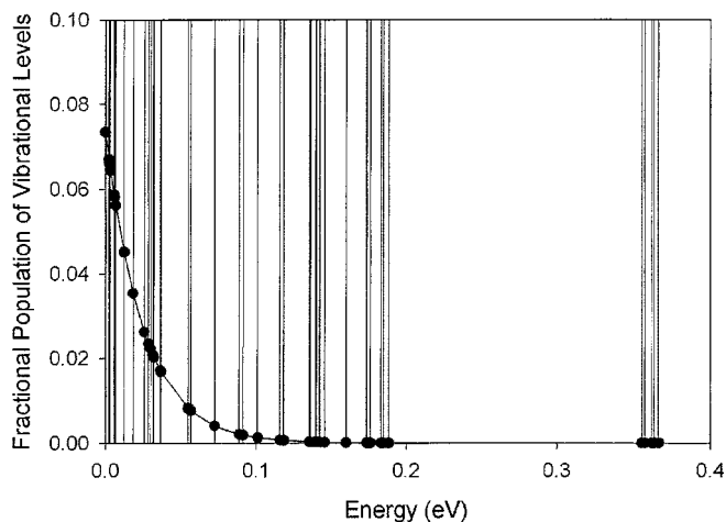
FIG. 4. The 94 lowest vibrational energies of TEOS. The solid circles show the fractional populations of the vibrational states at a temperature of 300 K.
