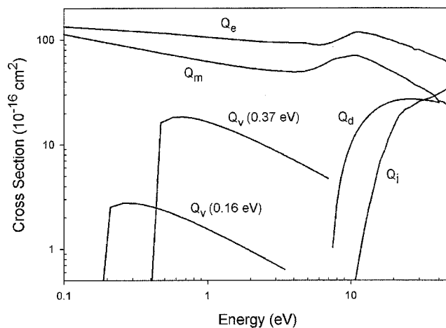
FIG. 5. Cross section set for TEOS. Q_e and Q_m are the integrated ab initio cross sections described in Sec. II.
